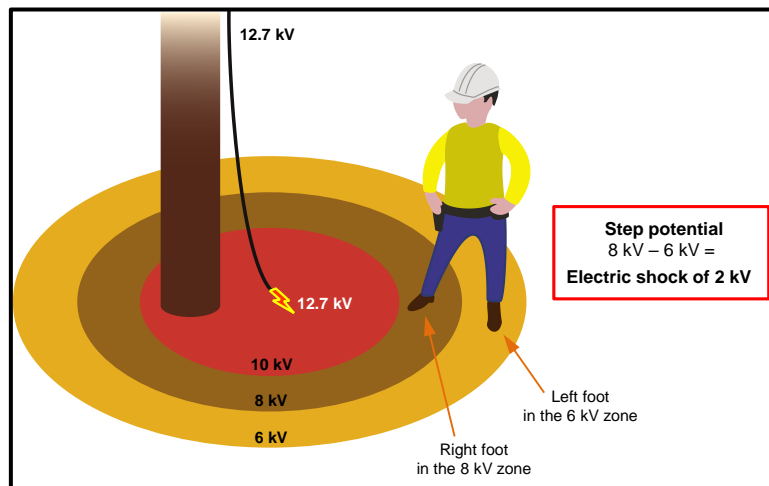
Figure 2 - Step potential
