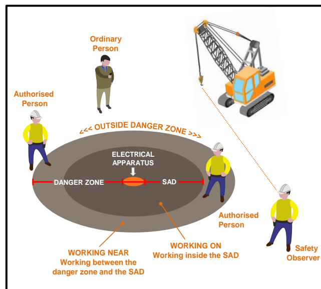
Figure 1 - Working on or near uninsulated electrical apparatus
