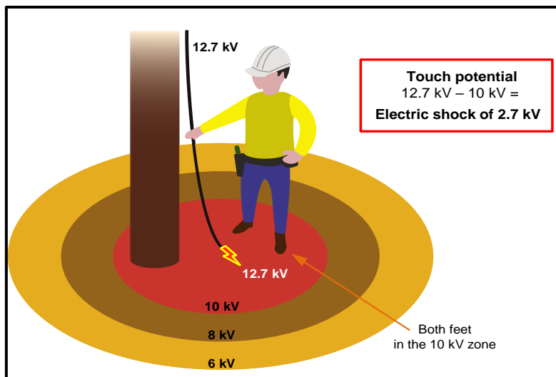
Figure 3 - Touch potential
